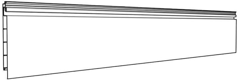
6" CrownWall™ Panel 48" +/- 1/4" (122 cm +/- 0.6cm) 8 Pieces
